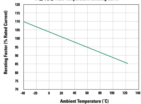
AB19U Fuse Temperature Derating Curve
